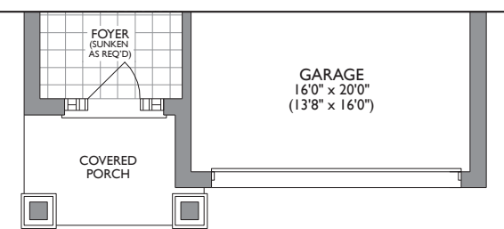
PARTIAL MAIN LEVEL ELEV. C
