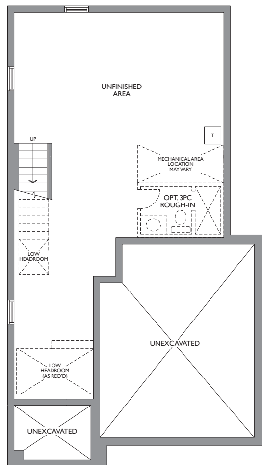
LOWER LEVEL ELEV. A, B & C
