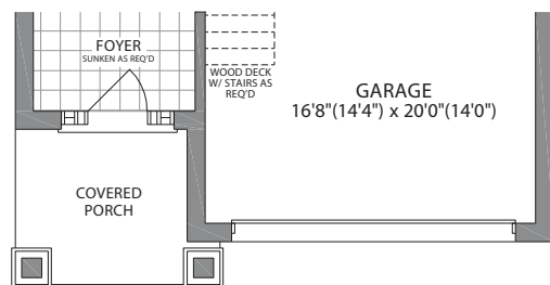
PARTIAL MAIN LEVEL ELEVATION A & C
