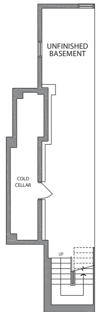
PARTIAL LOWER LEVEL ELEVATION A
