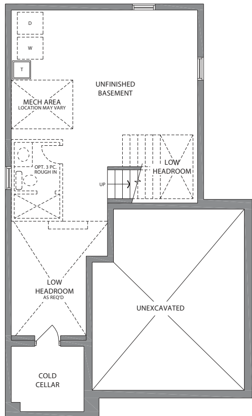
LOWER LEVEL ELEVATION A, B, & C
