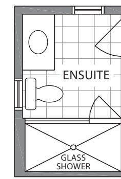
PARTIAL OPT. ENSUITE LAYOUT ELEVATION A
