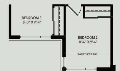
PARTIAL UPPER LEVEL
