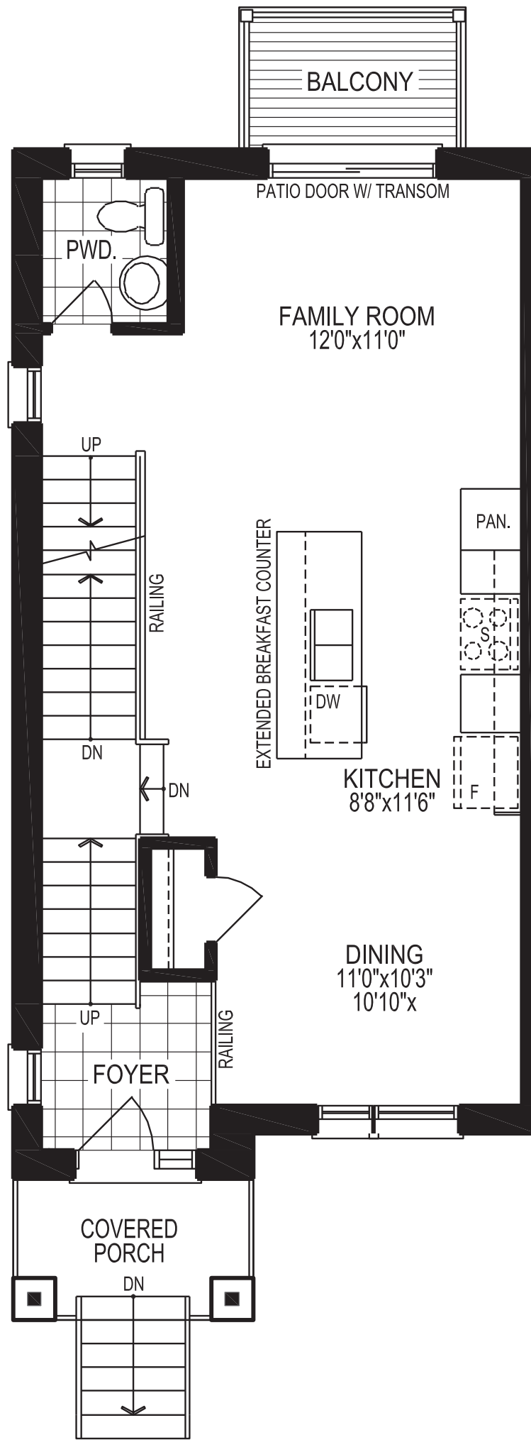
MAIN LEVEL ELEV. A
