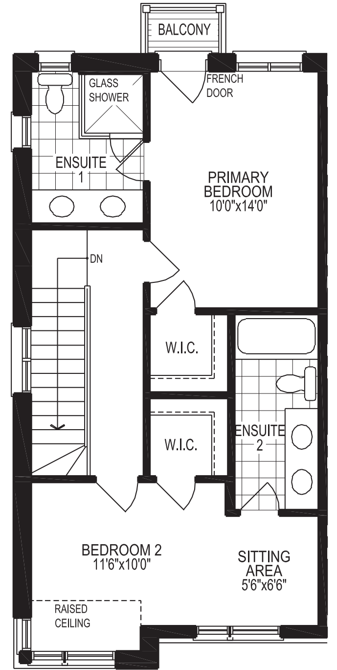
OPT. 2 BEDROOM UPPER LEVEL ELEV. A
