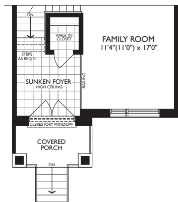
PART. MAIN LEVEL - ELEV. B
