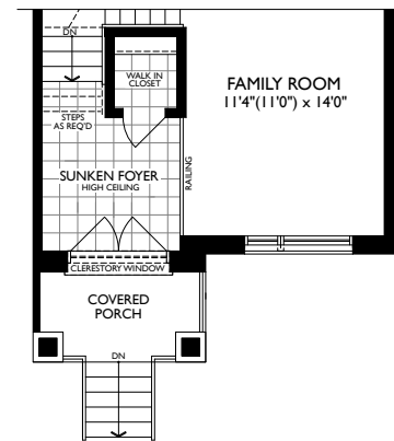
PART. OPT. MAIN LEVEL - ELEV. B
