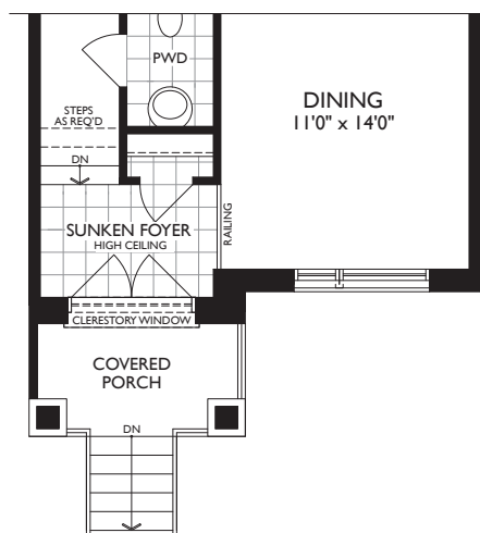
PART. MAIN LEVEL - ELEV. B
