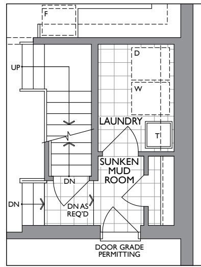
PARTIAL MAIN LEVEL OPT. 4 BEDROOM ELEV. A, B, & C
