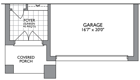
PARTIAL MAIN LEVEL ELEV. C
