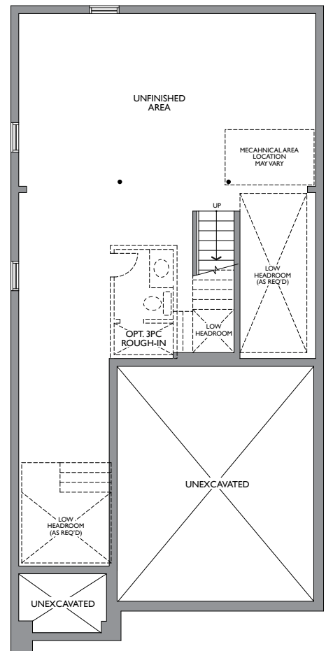
LOWER LEVEL ELEV. A
