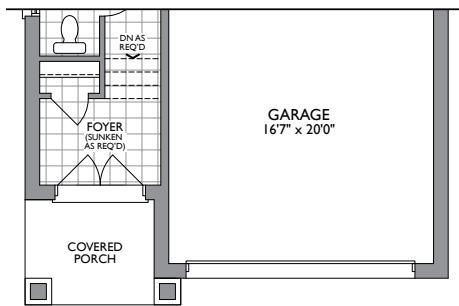
PARTIAL MAIN LEVEL ELEV. B & C
