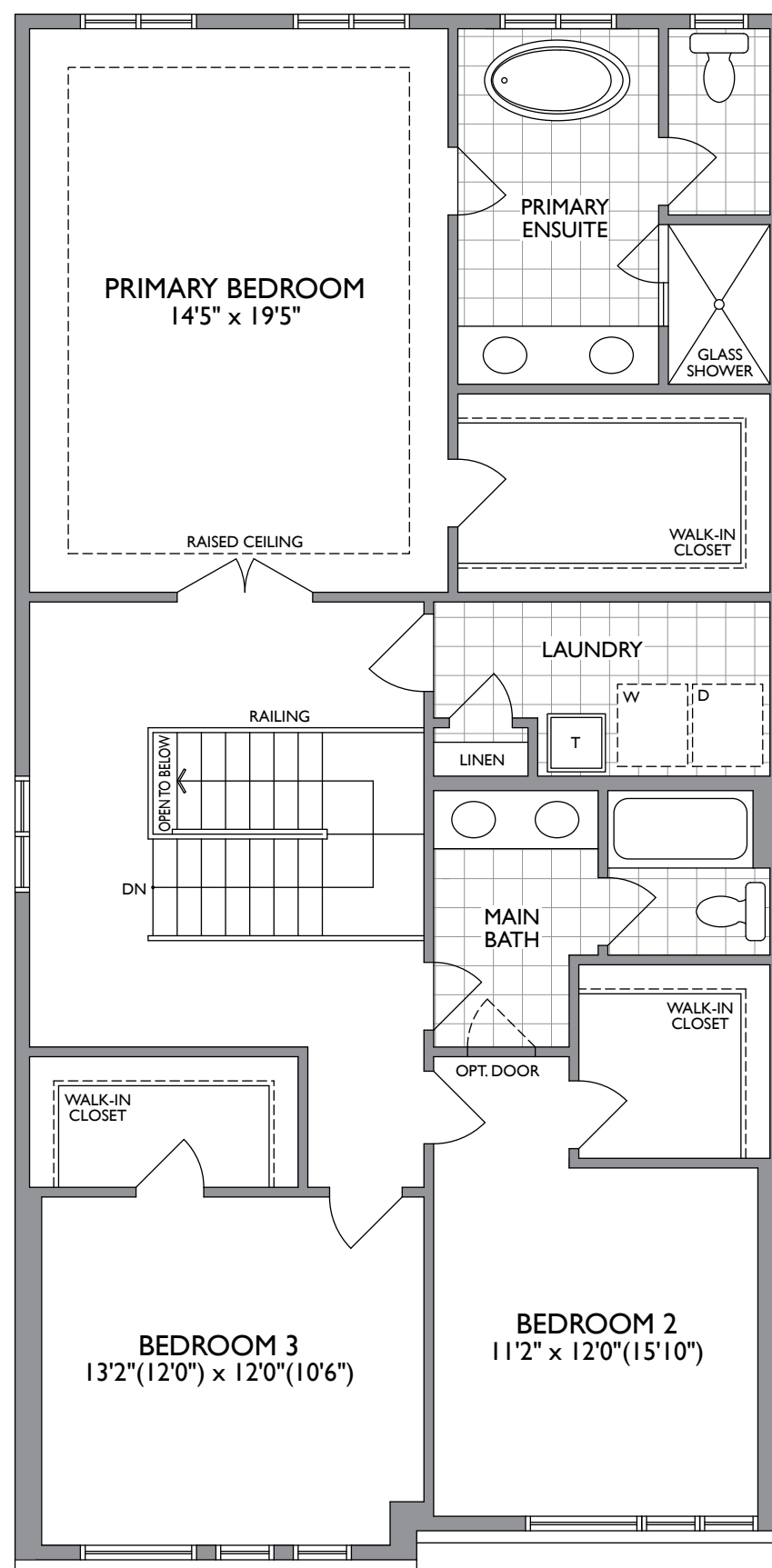
UPPER LEVEL ELEV. A
