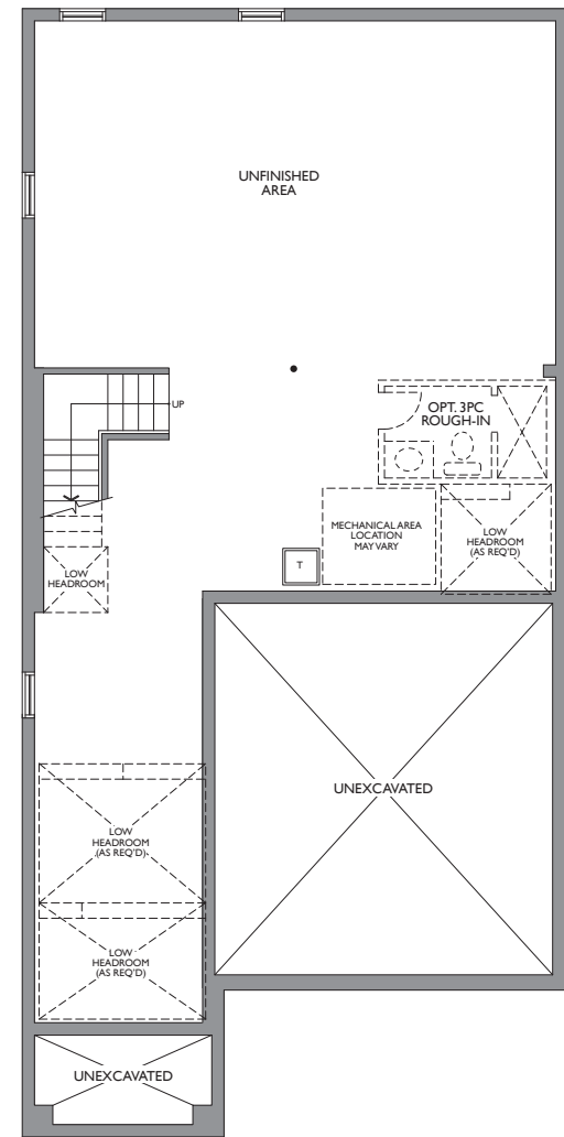
LOWER LEVEL ELEV. A & B
