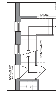
PARTIAL MAIN LEVEL WITH OPT. SIDE DOOR ELEV. A, B & C
