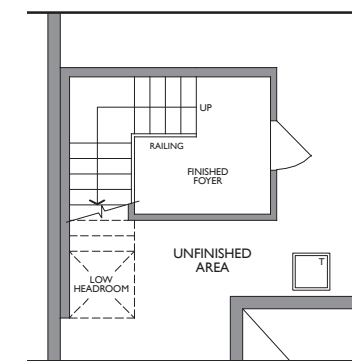
PARTIAL LOWER LEVEL WITH SIDE DOOR ENTRY ELEV. A, B & C
