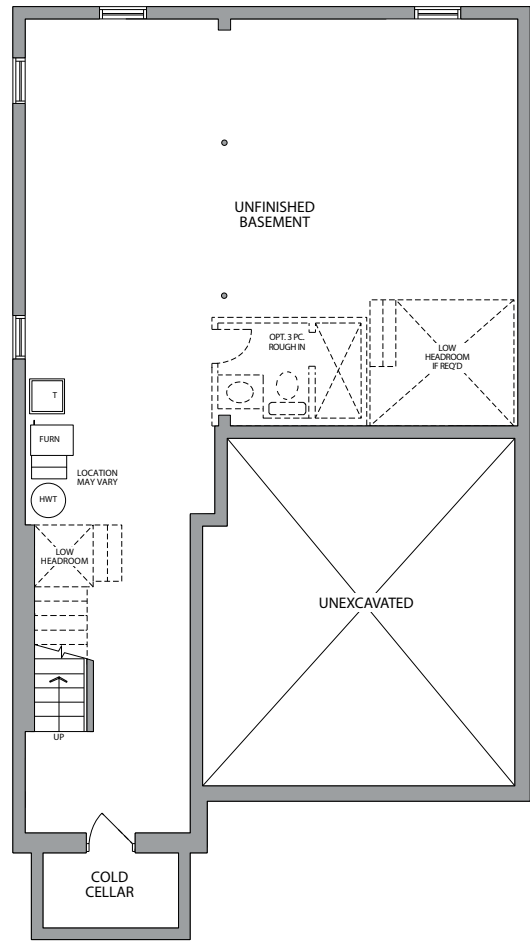
LOWER LEVEL ELEVATION C
