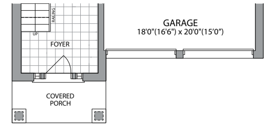
PARTIAL MAIN LEVEL ELEVATION D
